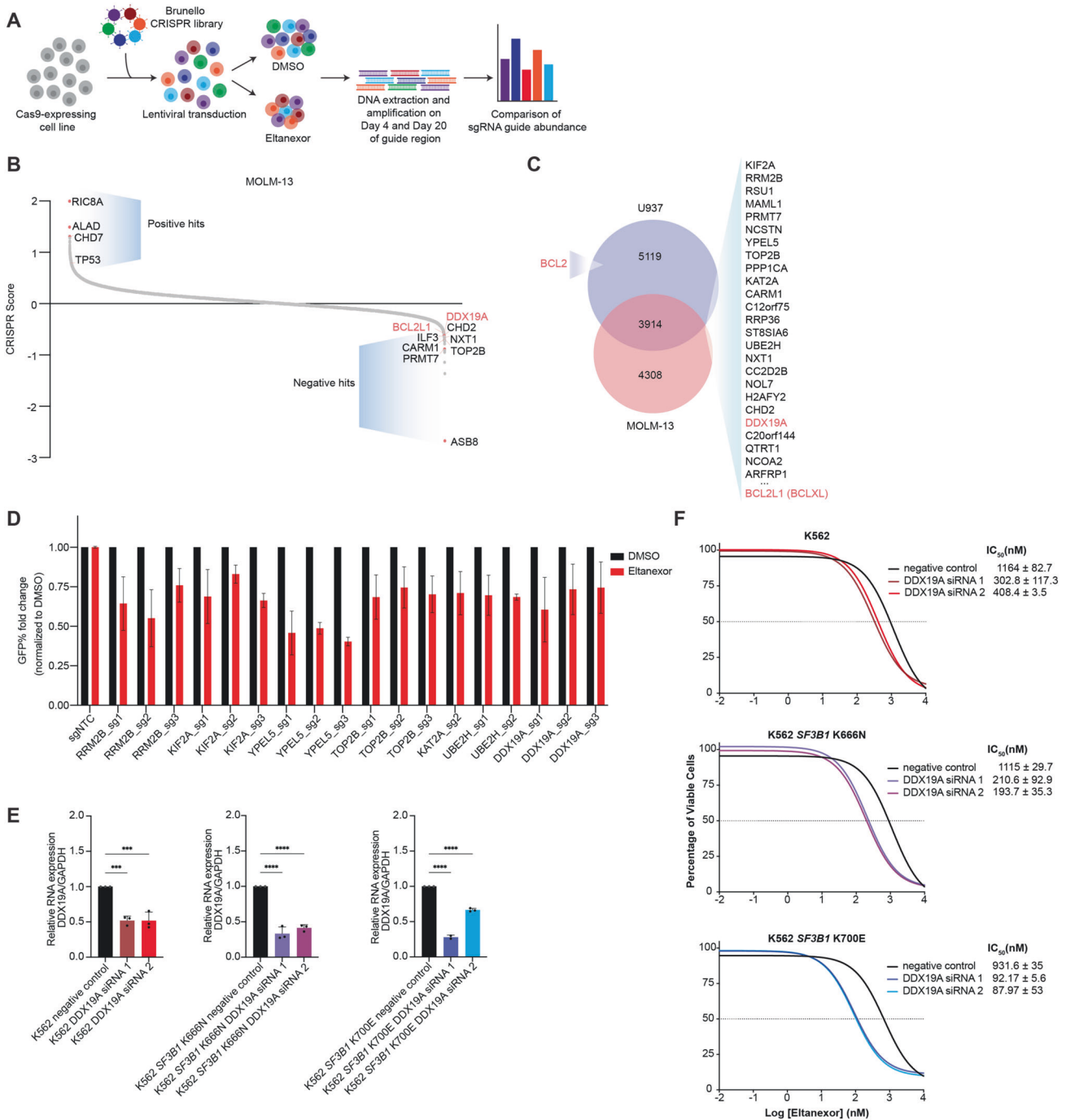
Fig. 4 CRISPR screen identified genes that may be associated with response to XPO1 inhibition. A Schematic of the Brunello genome-wide CRISPR screen in AML cell line, MOLM-13 cells treated with eltanexor. B Genome-wide CRISPR screen of MOLM-13 cells. Colored dots indicate genes involved in BCL2 pathway. CRISPR score represents the log 2 (fold-change) values of sgRNAs enriched (positive values) or depleted (negative values) after eltanexor treatment normalized to DMSO at Day 20 post-transduction. C Venn diagram of negative hits (sensitizers) in MOLM-13 and U937 CRISPR screens. D Competition-based assay of sgRNAs into MOLM-13 cells and treated with eltanexor for 48 h. Data is shown as mean + SEM. E RT-qPCR of DDX19A normalized to housekeeping gene GAPDH after 48 h of DDX19A siRNA-mediated gene silencing in K562 cells. F Dose-response curves of DDX19A siRNA knockdown cells treated with eltanexor for 48 h ( n = 3 replicates).
